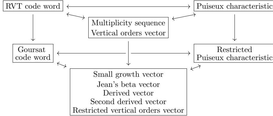
FIGURE 1. The invariants listed in the top five boxes were studied in our prior paper [2]; those listed in the bottom box are invariants of the small growth sequence of a Goursat germ. See Figure 2 for an example.
