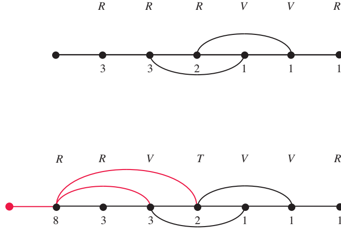
FIGURE 3. Obtaining the proximity diagram for the Goursat word RRVTVVR from the proximity diagram for its lifted Goursat word RRRVVR ; the new multiplicity is m_1 = 3 + 3 + 2 .
